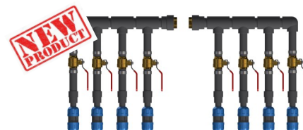
HDPE Design (FPT x Compression Connections) Main - FPT Fittings Circuits - Compression Fittings
