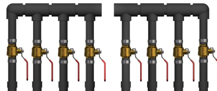
HDPE Design (Socket Fusion Connections) Main - Socket Fusion Circuits - Socket Fusion
